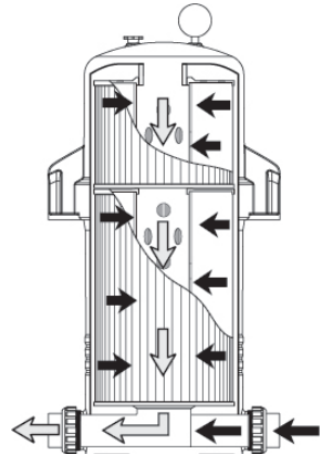
FLOW DIAGRAM
