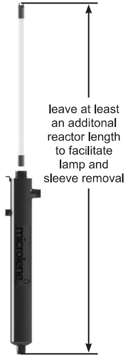
Figure 2. Lamp Removal Spacing
