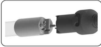
Figure 9a. Standard Output UV Lamp Connection
