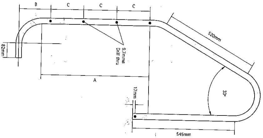
Standard Pool Ladder Rail All QR = 157mm
