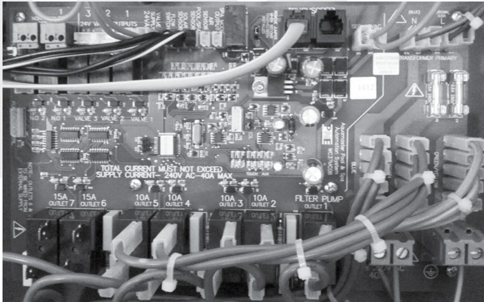
Aquamaster Control PCB image
