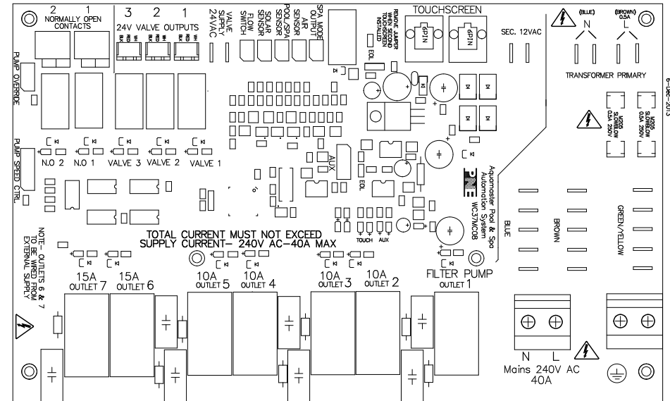
Aquamaster Control PCB layout
