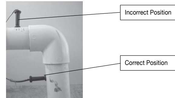
Pool Sensor Installation
